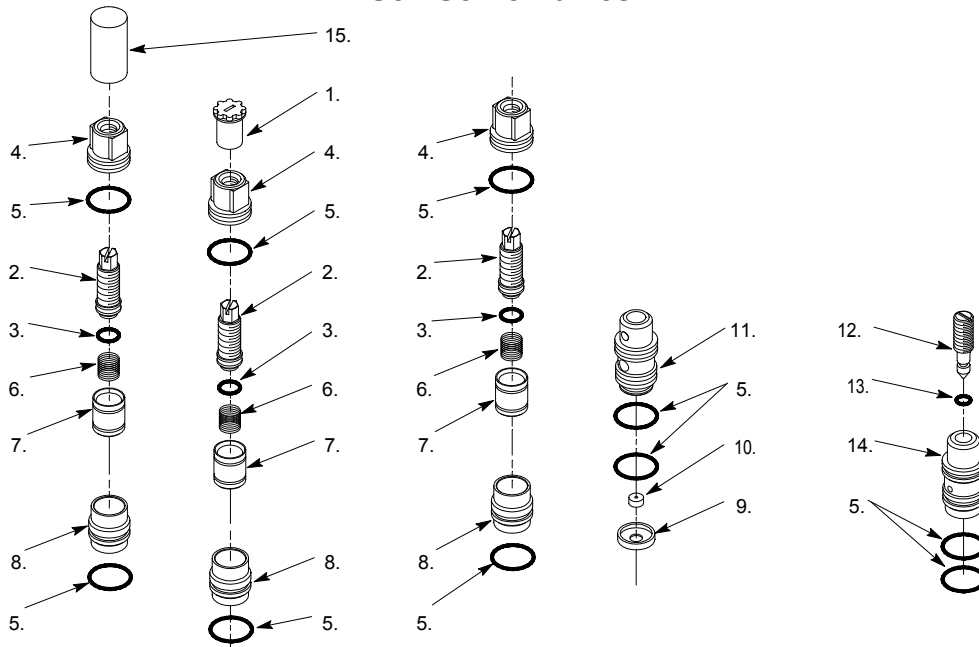
FAST FLOW VALVE
