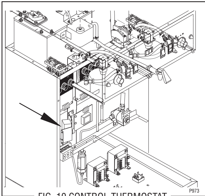
FIG. 10 CONTROL THERMOSTAT
