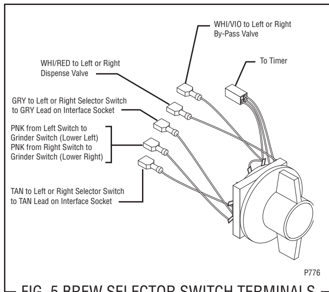
FIG. 5 BREW SELECTOR SWITCH TERMINALS
