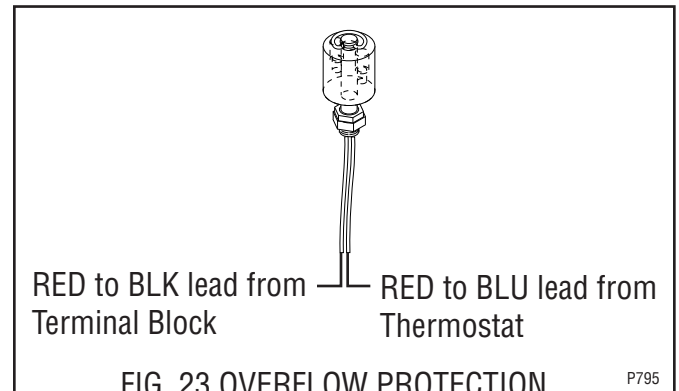
FIG. 23 OVERFLOW PROTECTION SWITCH LEADS
