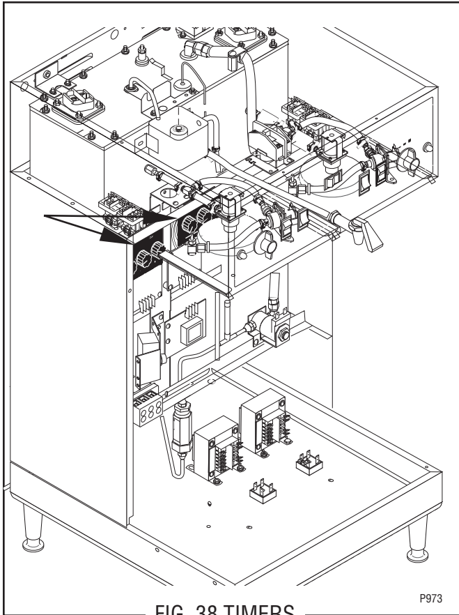
FIG. 38 TIMERS
