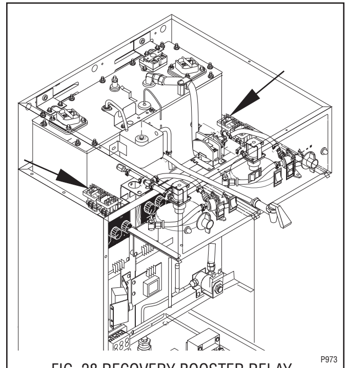
FIG. 28 RECOVERY BOOSTER RELAY
