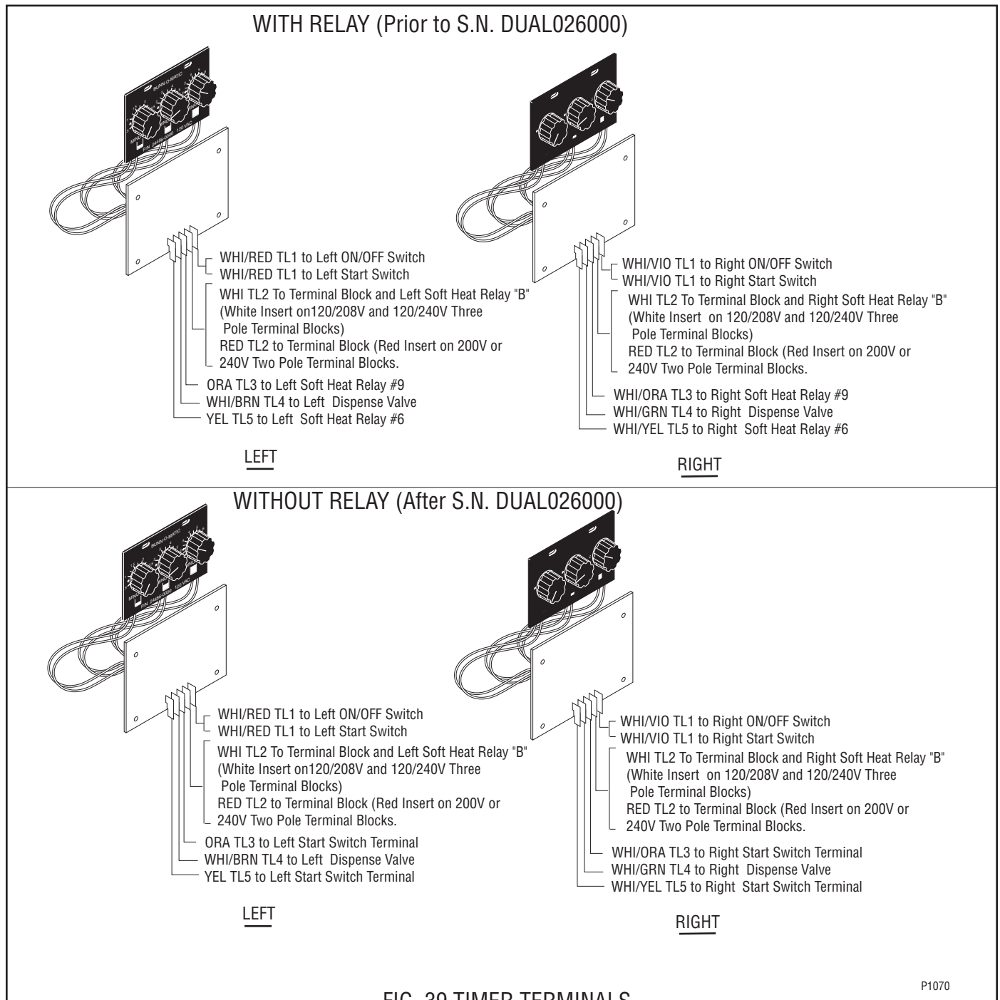
FIG. 39 TIMER TERMINALS
