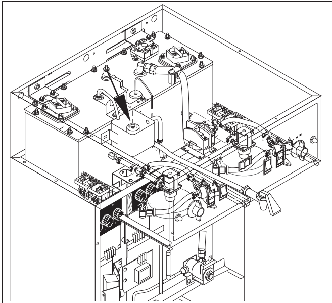
FIG. 22 OVERFLOW PROTECTION SWITCH
