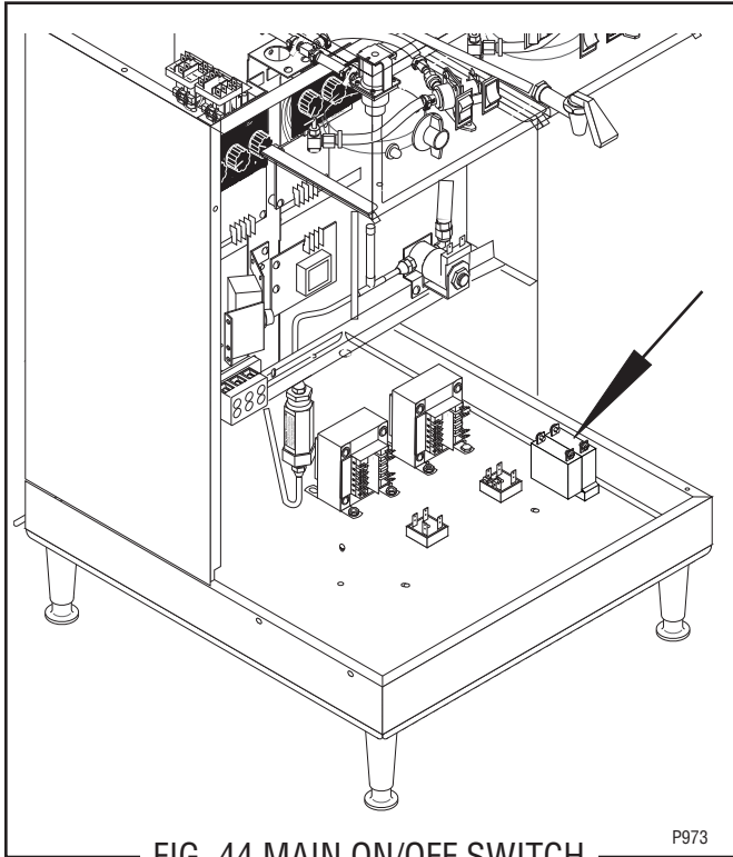
FIG. 44 MAIN ON/OFF SWITCH
