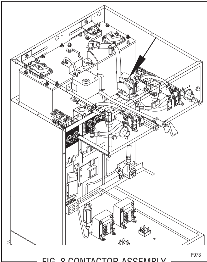
FIG. 8 CONTACTOR ASSEMBLY
